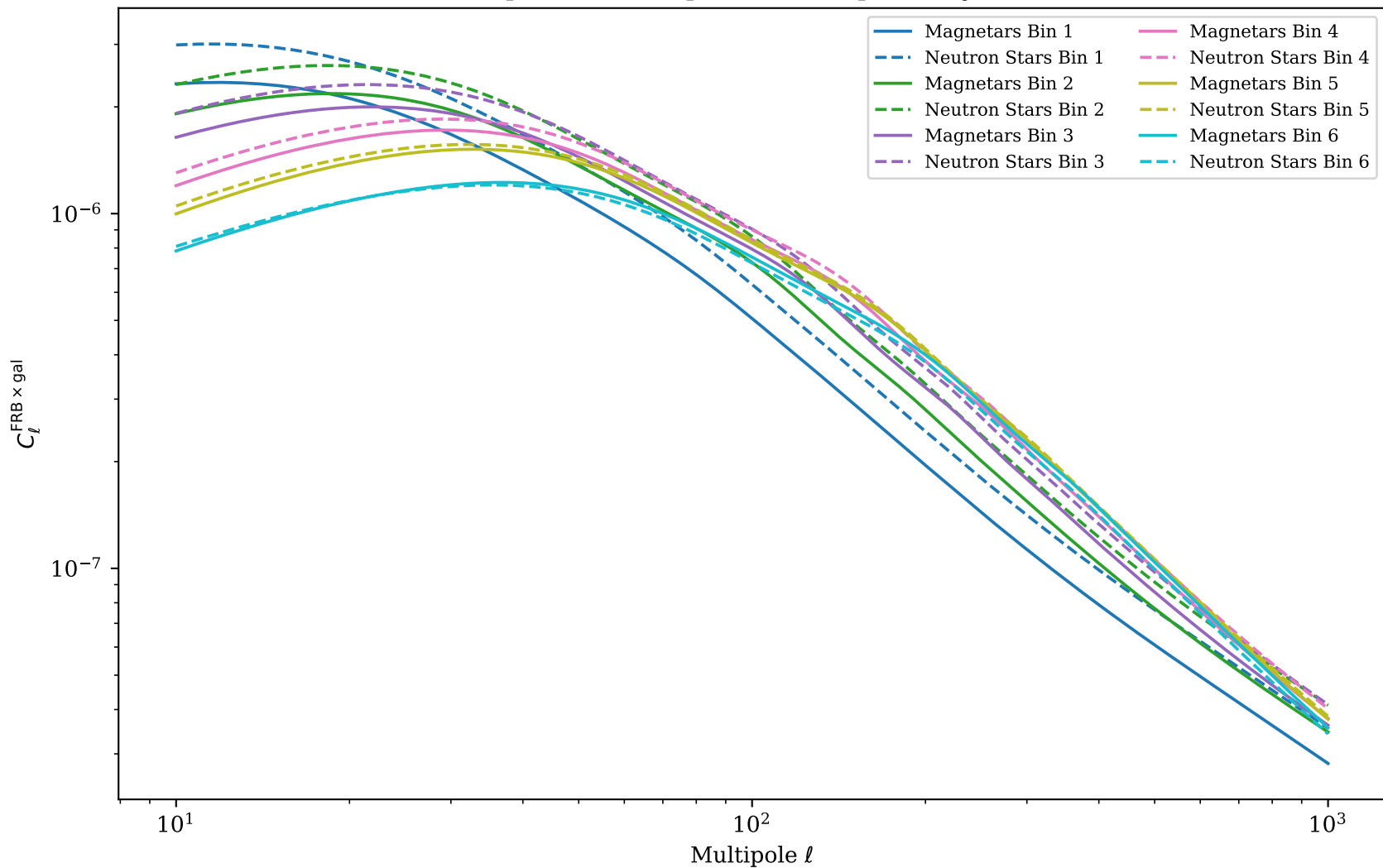
FRB Population Comparison (Deep Survey, all bins)
